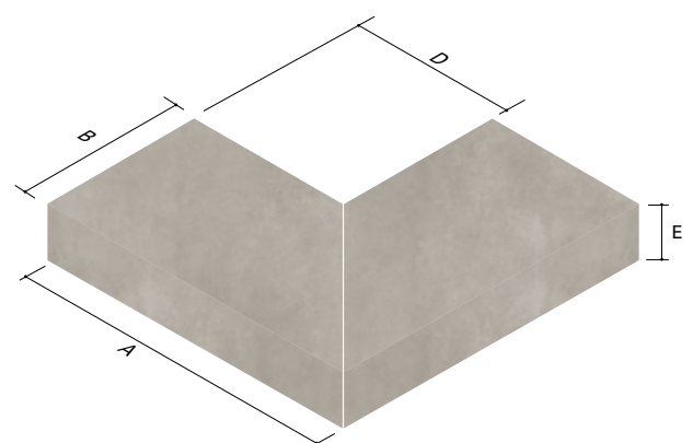
Nosing tile - outside corner
